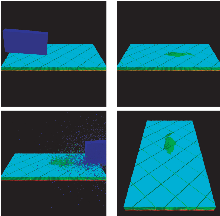
Fig. 2 Simulation results for case MLGD 2.
